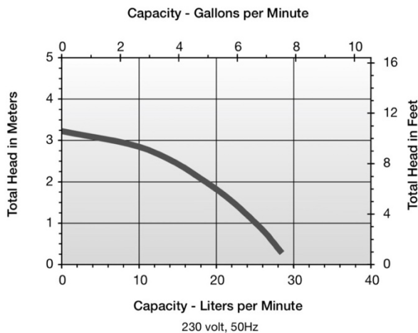
Performance Curves 2-MD-HC 230V, 50/60Hz
