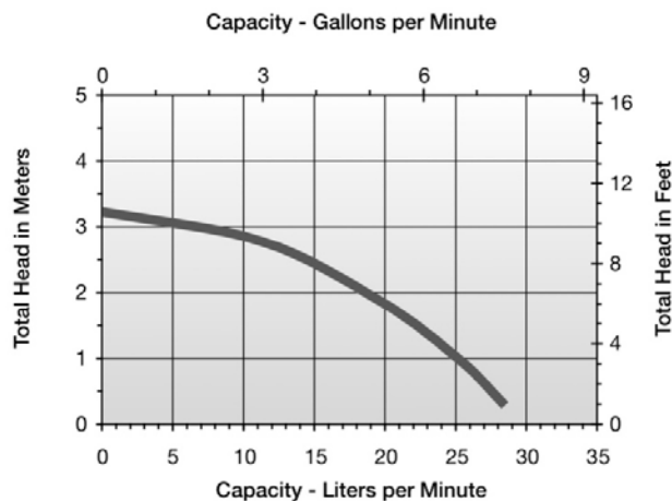
Performance Curves 2-MD 230V, 50/60Hz
