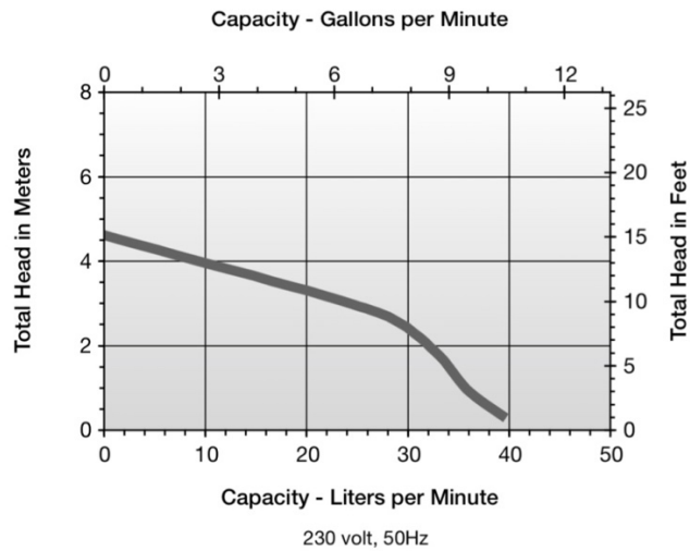
Performance Curves 3-MD-SC 230V, 50Hz
