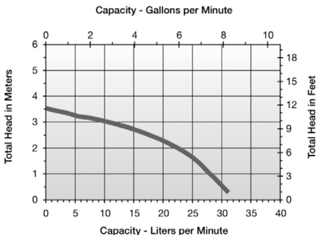
Performance Curves TE-3-MD 230V, 50/60Hz
