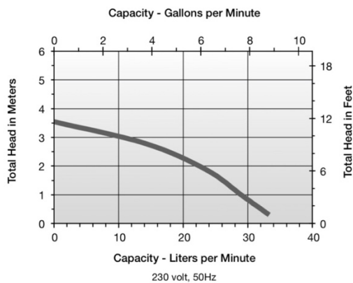
Performance Curves TE-3-MD-SC 230V, 50/60Hz
